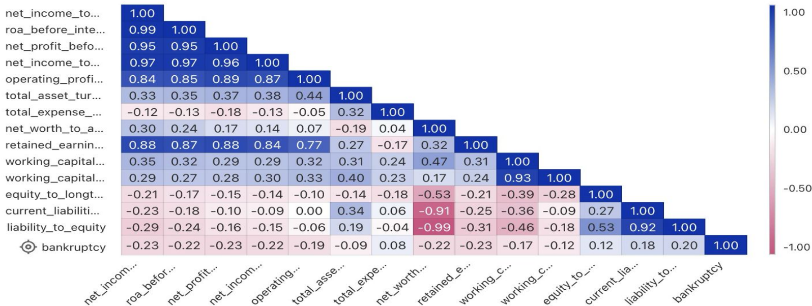
Correlation Matrix
